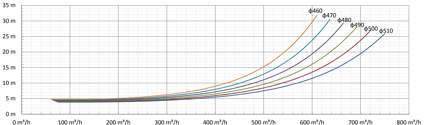
NPSH [m]
